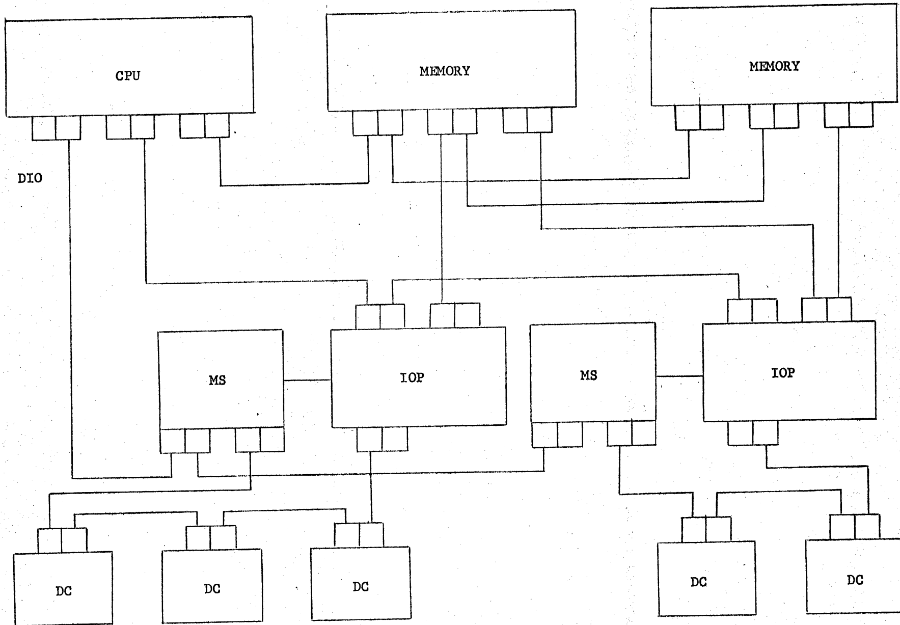
FIG. 2.1 SYSTEM DIAGRAM
